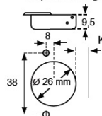
Cup drawing
